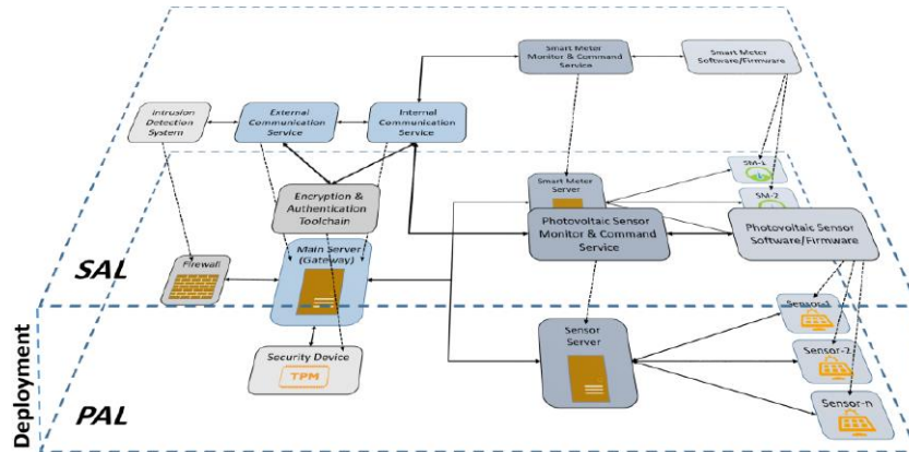
Fig. 4. PAL, SAL and deployment sub-models of the CTTP model of a smart metering system.
