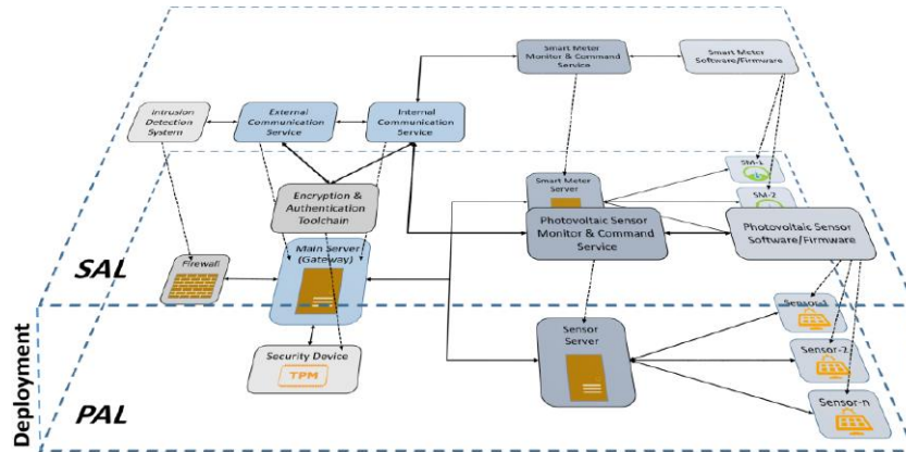
Fig. 4. PAL, SAL and deployment sub-models of the CTTTP model of a smart metering system.
