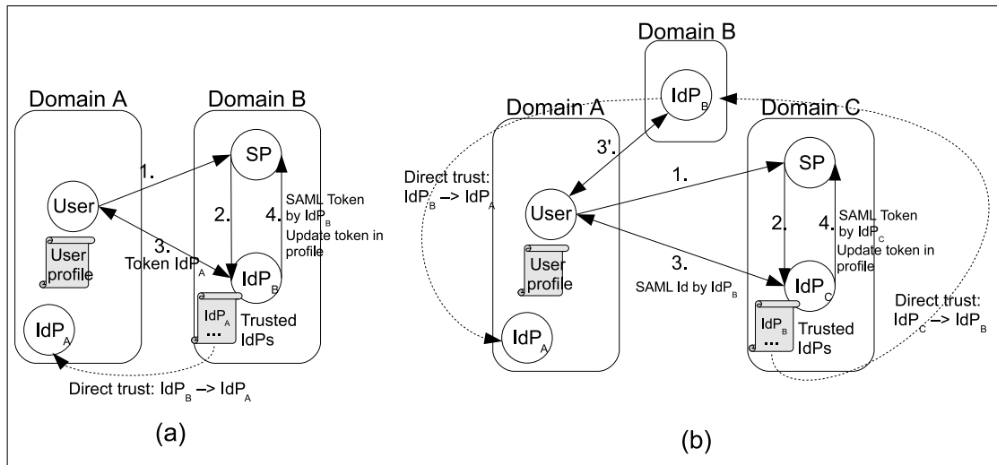
Fig. 7. User profile evolution scenario
