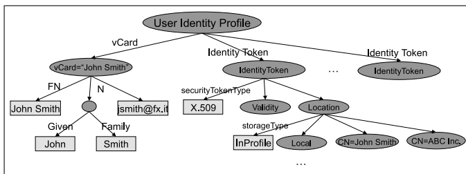
Fig. 4. User profile example
