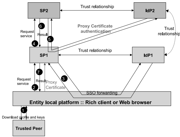
Fig. 3. Service composition using proxy certificates
