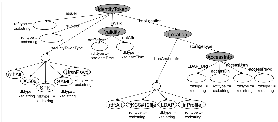
Fig. 5. User profile identity token schema: an RDF graph
